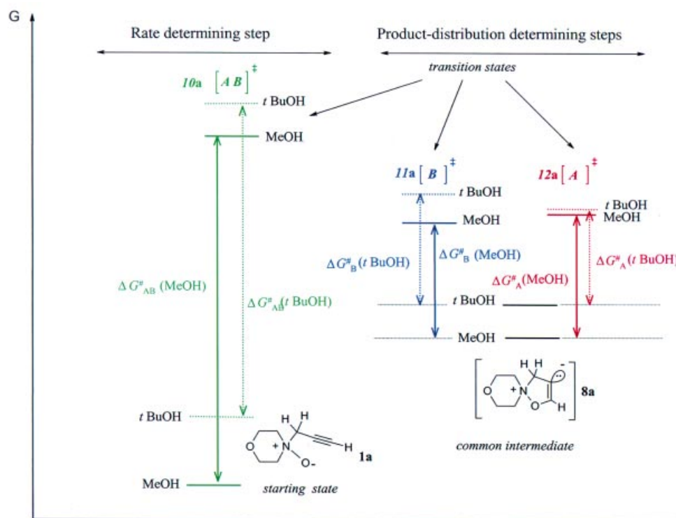
Scheme 6. Schematic energy level diagram: solvent dependence of the rate-determining step and of the product distribution determining steps of the rearrangements
