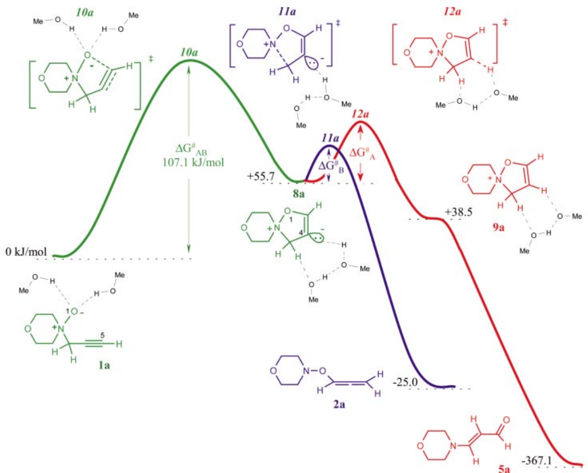
Scheme 5. Energy profile of the competing reactions in protic medium based on ab initio calculations
