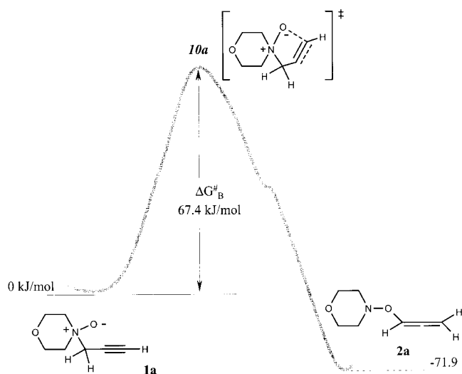
Scheme 4. Energy profile of route B' in aprotic medium, based on ab initio calculations
