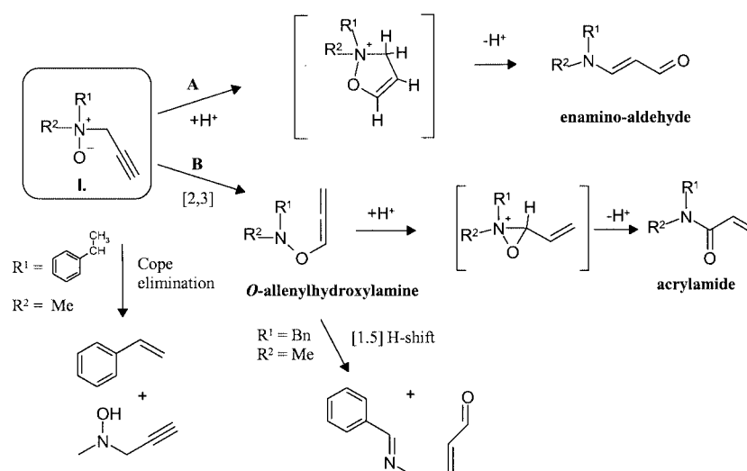
Scheme 1. Possible rearrangements of tertiary propargylamine N -oxides
