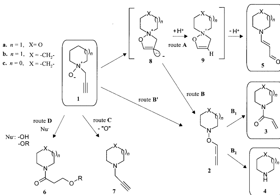
Scheme 3. Competing reaction routes of cyclic tertiary propargylamine N -oxides
